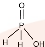
Hypophosphorous acid (Phosphinic acid) \text{H}_3\text{PO}_2 (monobasic)
