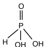
Hypophosphorous acid (Phosphinic acid) \text{H}_3\text{PO}_2 (monobasic)
